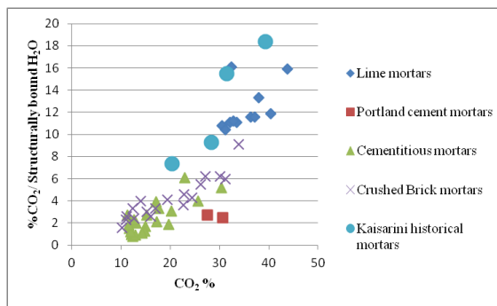
Figure 5: Grouping of the Kaisiriani mortars according to thermal analysis results
